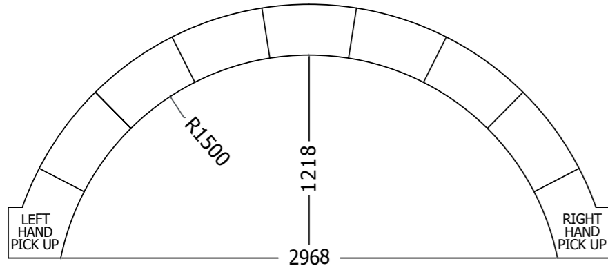
5FT LOW PROFILE ROMAN END BAY (Country leisure 12ft roman end bay) (finished wall to wall measurements)
