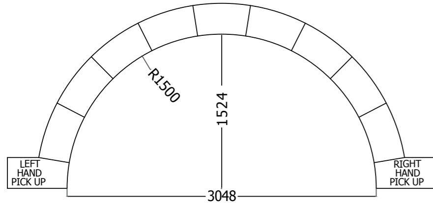
5FT ROMAN END BAY (finished wall to wall measurements)
