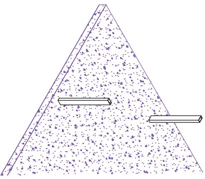
STAGE 3 When mesh is in position, pour concrete into excavation to cover mesh by 50mm minimum.
